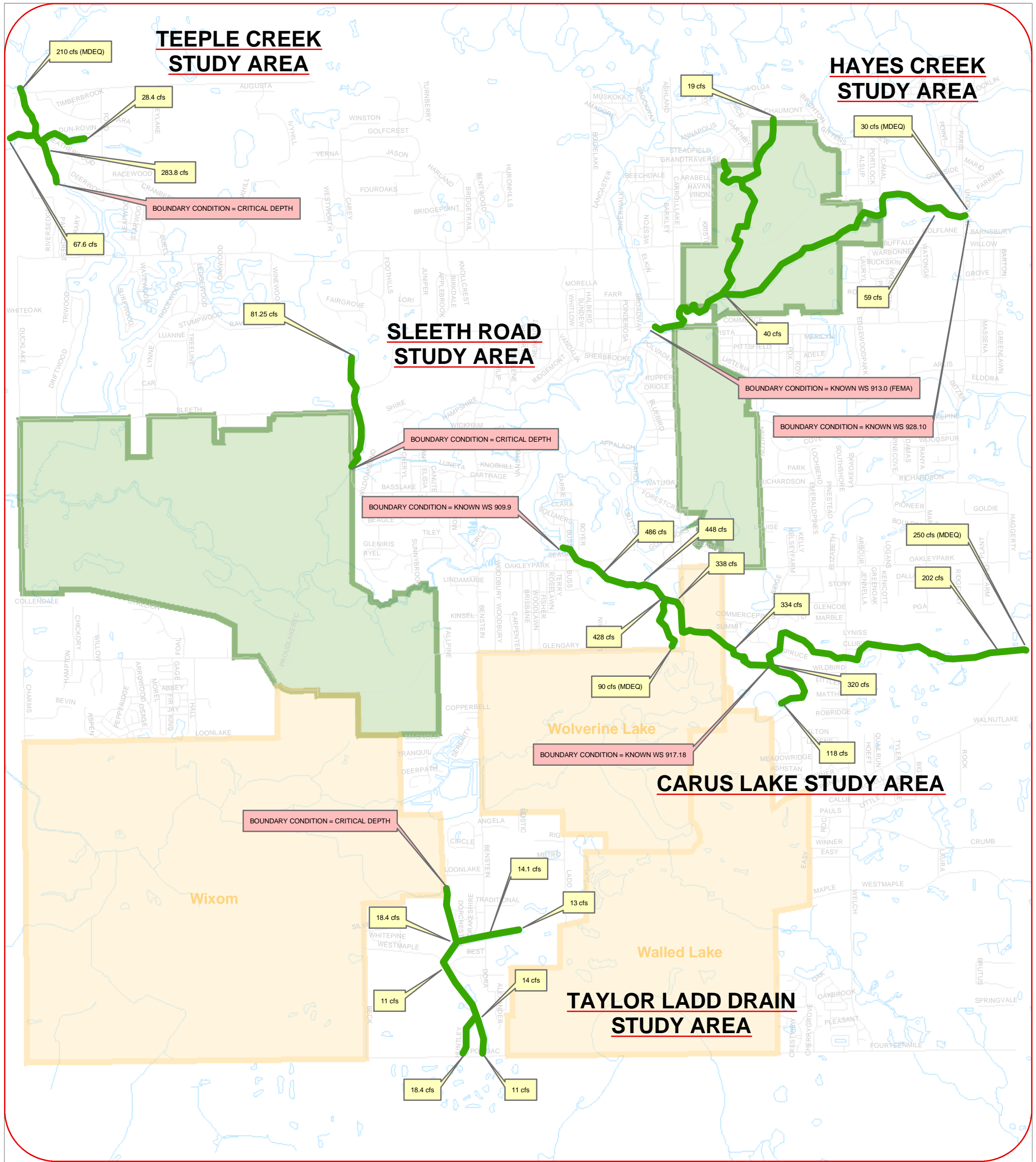
Flow Boundary Conditions and Locations
